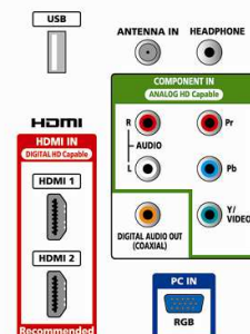
Rear Panel
